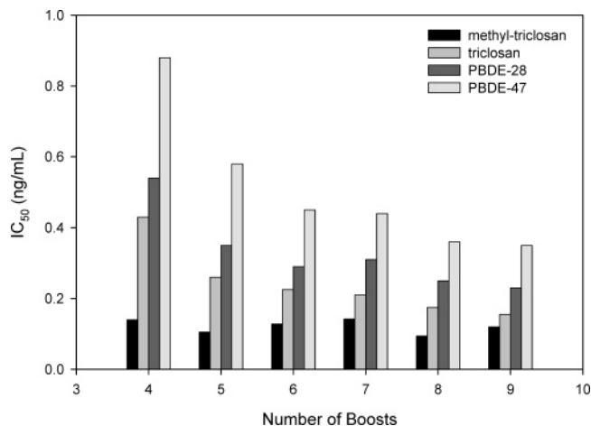
Figure 2. Change in \text{IC}_{50} of various substrates with an increased number of booster immunizations.
